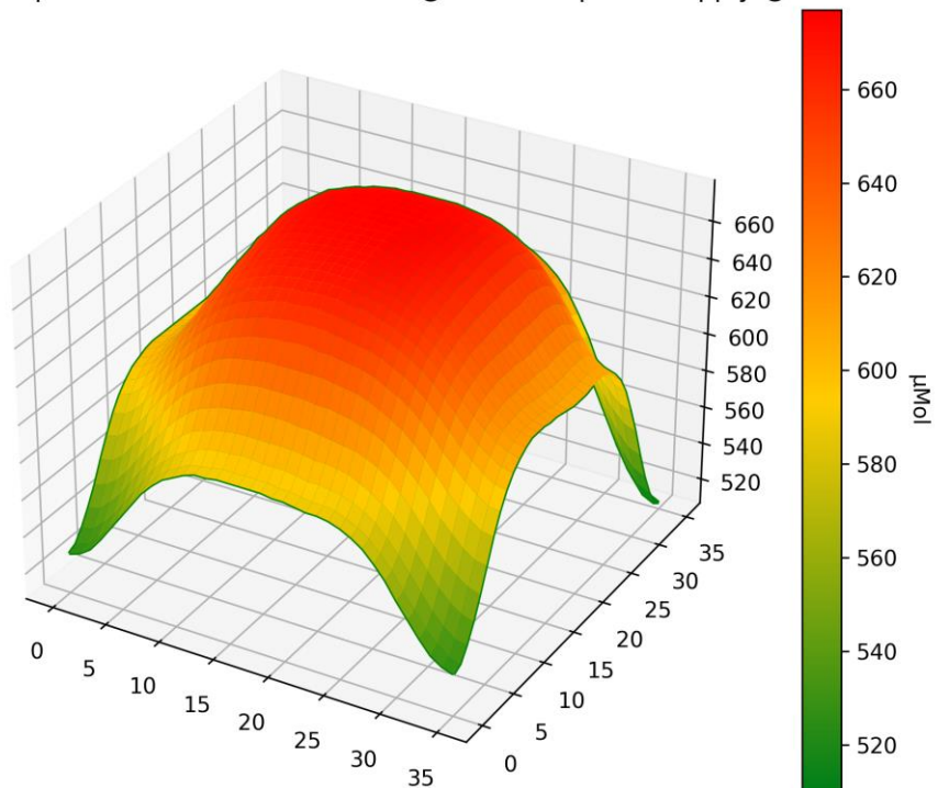
PPFD 3D Heatmap LT-3691 - 6500K - Distance @ 600mm - power supply @ 3500mA
