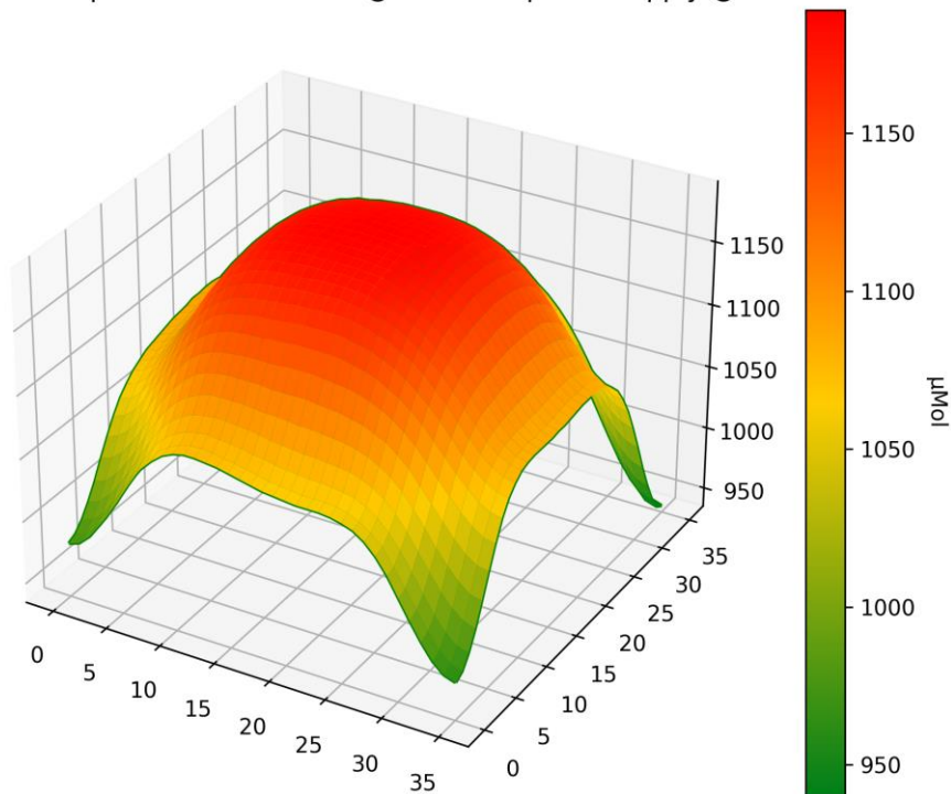
PPFD 3D Heatmap LT-4770 - Distance @ 600mm - power supply @ 5710mA
