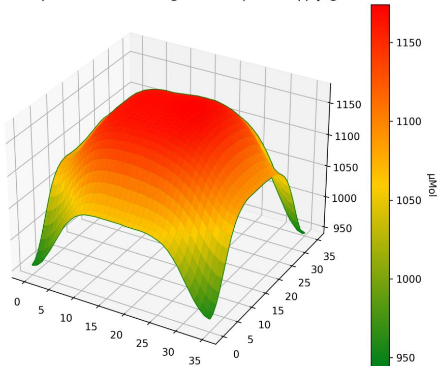
PPFD 3D Heatmap LT-4772 - Distance @ 600mm - power supply @ 5710mA
