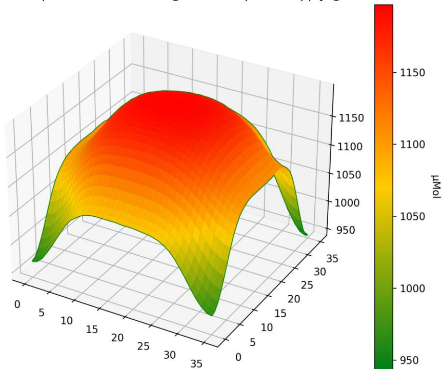
PPFD 3D Heatmap LT-4774 - Distance @ 600mm - power supply @ 5710mA
