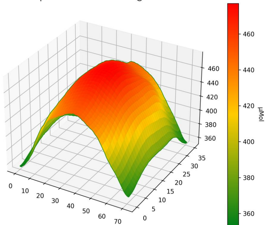
PPFD 3D Heatmap LT-5918 3500K+660nm @ 90cm - Power - 100%
